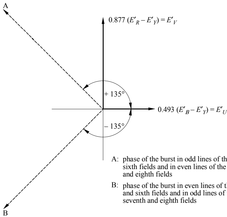
b) PAL system
