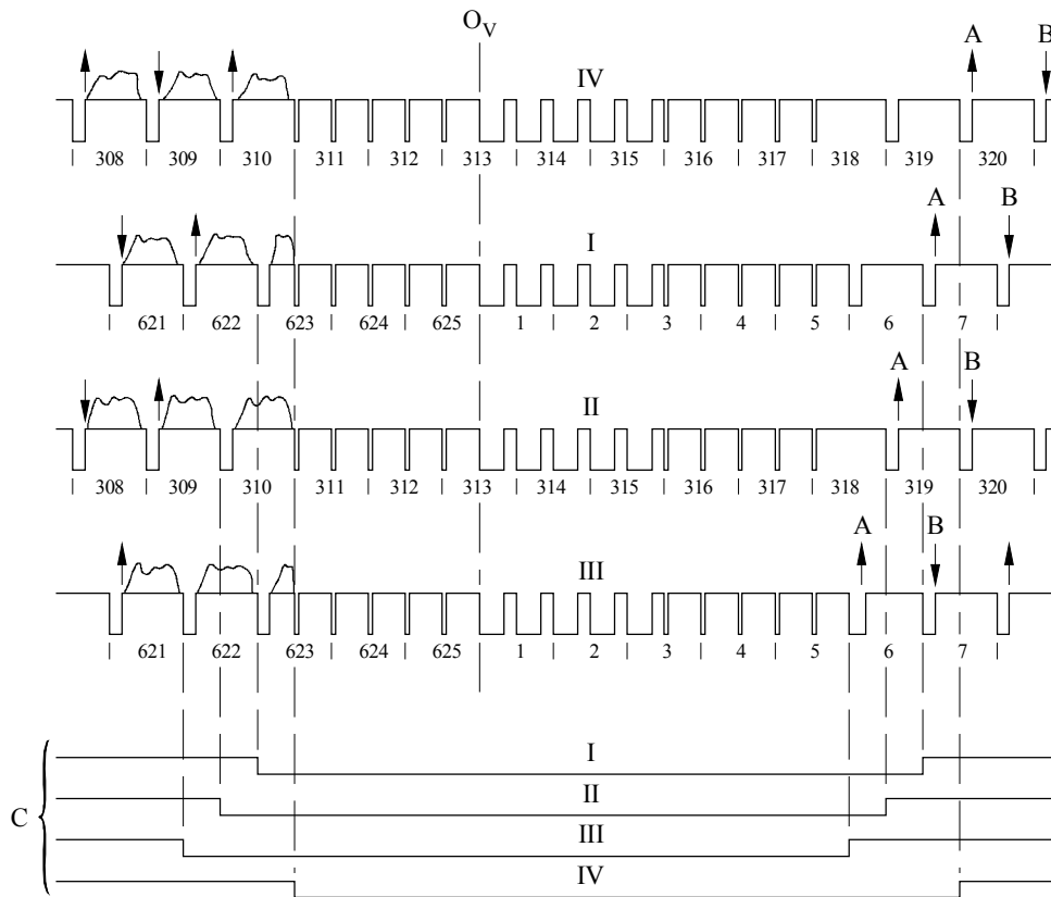
FIGURE 5a Burst-blanking sequence in the B, B1, D, D1, G, H, K and I/PAL systems
