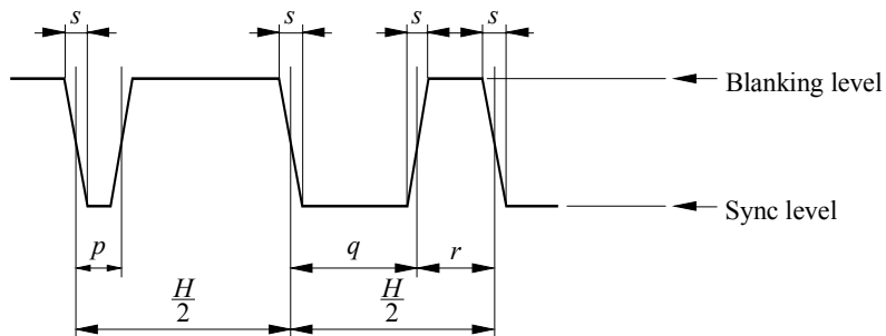
FIGURE 2-1c – Details of equalizing and synchronizing pulses
